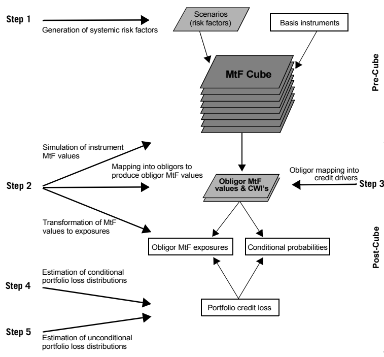
Figure 4: MtF framework for integrated market and credit risk
